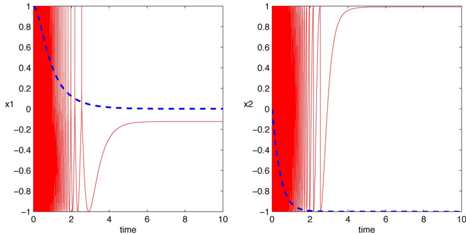
Fig. 3. Time histories of the states of the system (42) with p = 2, q = 1, \Psi(s) = |s|, \eta = 0 and x(0) = [1 \ 0 \ 1]' : k_1 = k_2 = 1 (blue/dashed); k_1 = 1000, k_2 = 1 (red/solid).
