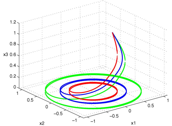
Fig. 1. The trajectory of system (42), with p = 2, q = 3, k_1 = k_2 = 1, \Psi(s) = |s|, x(0) = [0.5 \ 0 \ 1]^T , for the three considered cases. The trajectory converges to the circle of radius \rho_0 = 0.5 for \eta = 0 (red/dotted); of radius \min(1, \rho_0) \leq \rho \leq \max(1, \rho_0) for \eta = 1 and r = 4 (blue/solid); of radius 1 for \eta = 1 and r = 2 (green/dashed).
