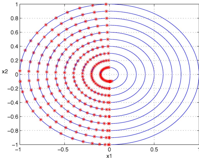
Fig. 4. Projection of the phase portrait on the (x_1, x_2) -plane for p = 2, q = 3, k_1 = k_2 = 1, \Psi(s) = |s| and \eta = 0 and the set of initial conditions \{(x_1(0), x_2(0), x_3(0)) : x_1(0)^2 + x_2(0)^2 \leq 1, x_3(0) = 1\} . The final states are represented by stars.
