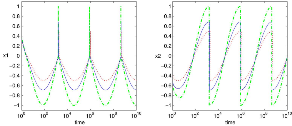
Fig. 2. Time histories of the states of the system (42) with p = 2, q = 3, k_1 = k_2 = 1, \Psi(s) = |s| and x(0) = [0.5 \ 0 \ 1]' : \eta = 0 (red/dotted); \eta = 1 and r = 4 (blue/solid); \eta = 1 and r = 2 (green/dashed).
