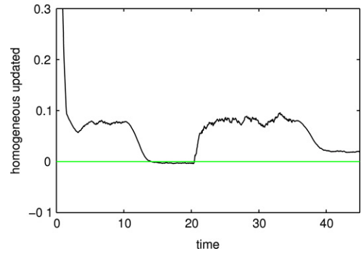
Fig. 2. Estimation error \eta_2 - \hat{\eta}_2 given by each observer.
