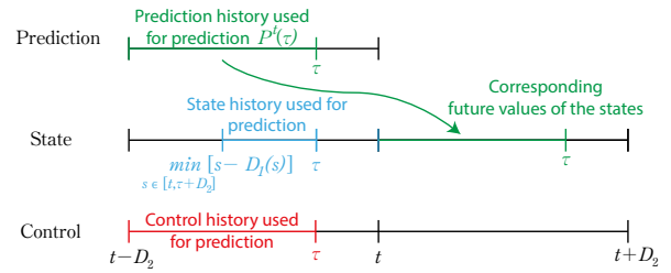
Fig. 1. Schematic view of the variables involved in the computation of the prediction P^t(\tau) in (12).
