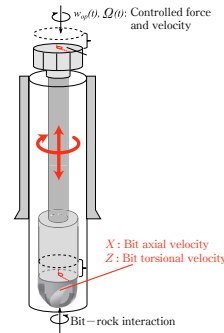
Fig. 3. Schematic view of drilling facilities.
